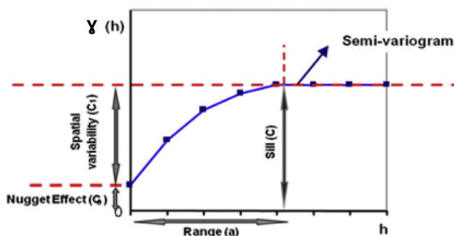
Fig. 3. Example of a variogram with ideal characteristics.
