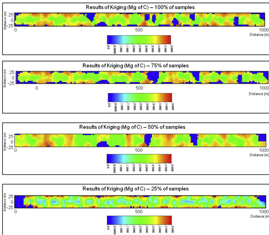
Fig. 15. Kriging results.
