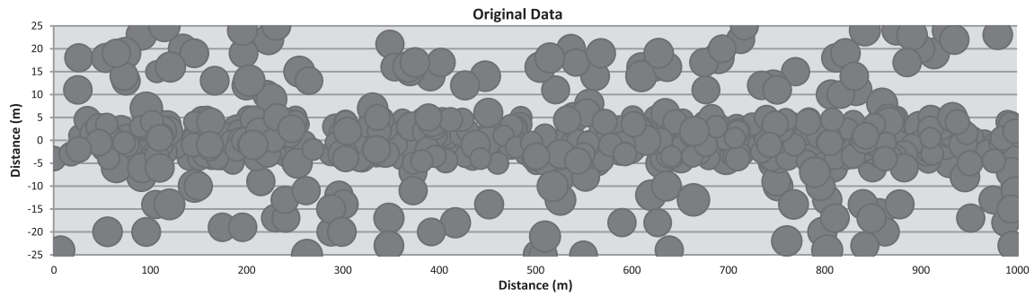
Fig. 6. Georeferenced samples.
