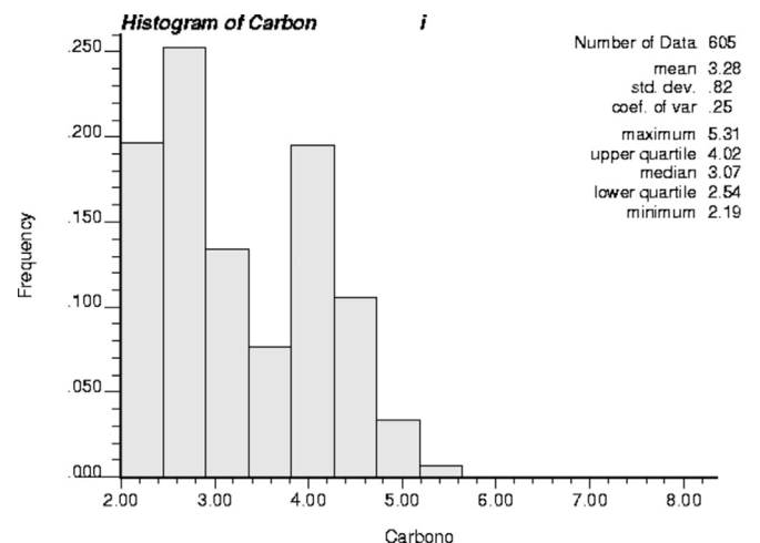
Fig. 9. Histogram of the frequency distribution of the carbon variable (Mg of C).
